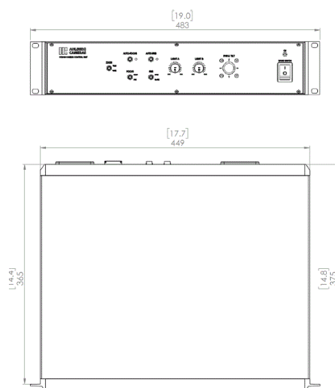
Figure 2 – CCU100 dimensions
